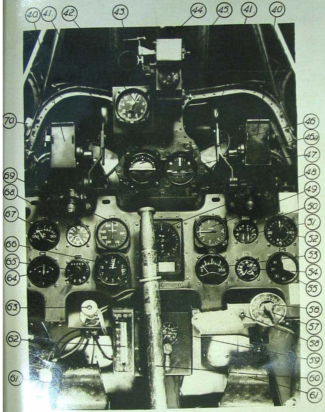
N° 7. Cockpit Front with Instrument Panel.
